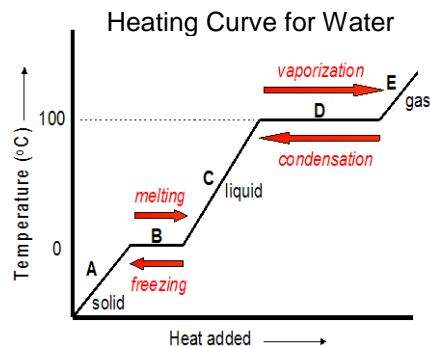
Energy Changes Accompanying Phase Changes
