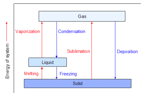
Energy Changes Accompanying Phase Changes
